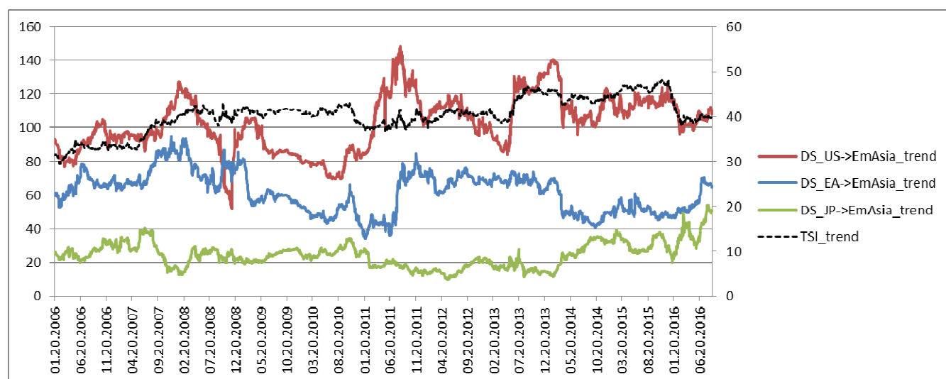
Figure A1: Dynamics of total spillover index and directional spillovers from major advanced countries to Emerging Asia: specification with included trend 17
