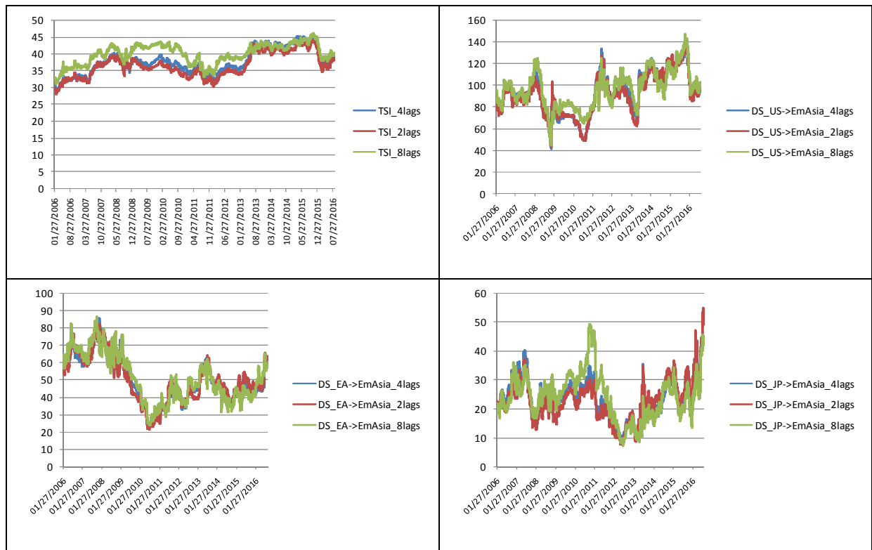
Figure 19: Sensitivity of the results to different lag order choices
