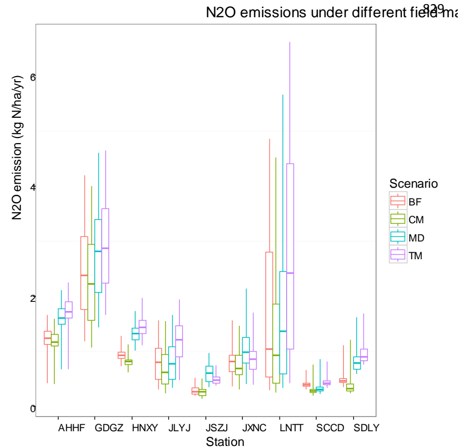
Figure 5. The boxplots of methane emission (left, denoted as Figure 5-a.) and nitrous oxide emission (right, Figure 5-b.) under field management scenarios of Traditional Management (TM), Balanced Fertilizer (BF), Midseason Drainage (MD) and Comprehensive Management (CM).
