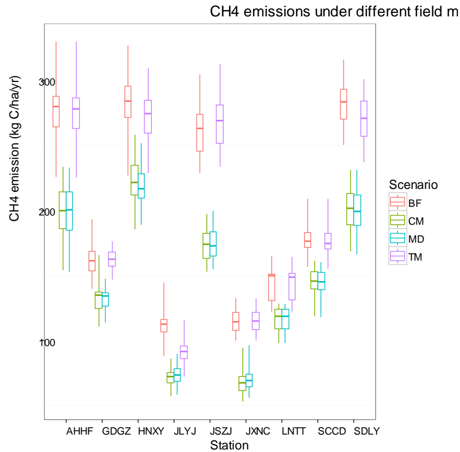
Figure 5. The boxplots of methane emission (left, denoted as Figure 5-a.) and nitrous oxide emission (right, Figure 5-b.) under field management scenarios of Traditional Management (TM), Balanced Fertilizer (BF), Midseason Drainage (MD) and Comprehensive Management (CM).
