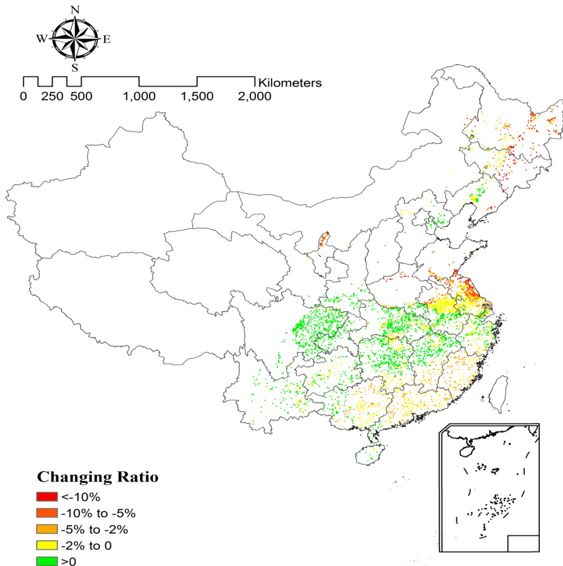
Figure 6. Changes of the simulated best attainable yields at the grid-cell level under the comprehensive mitigation scenario versus the traditional management scenario
