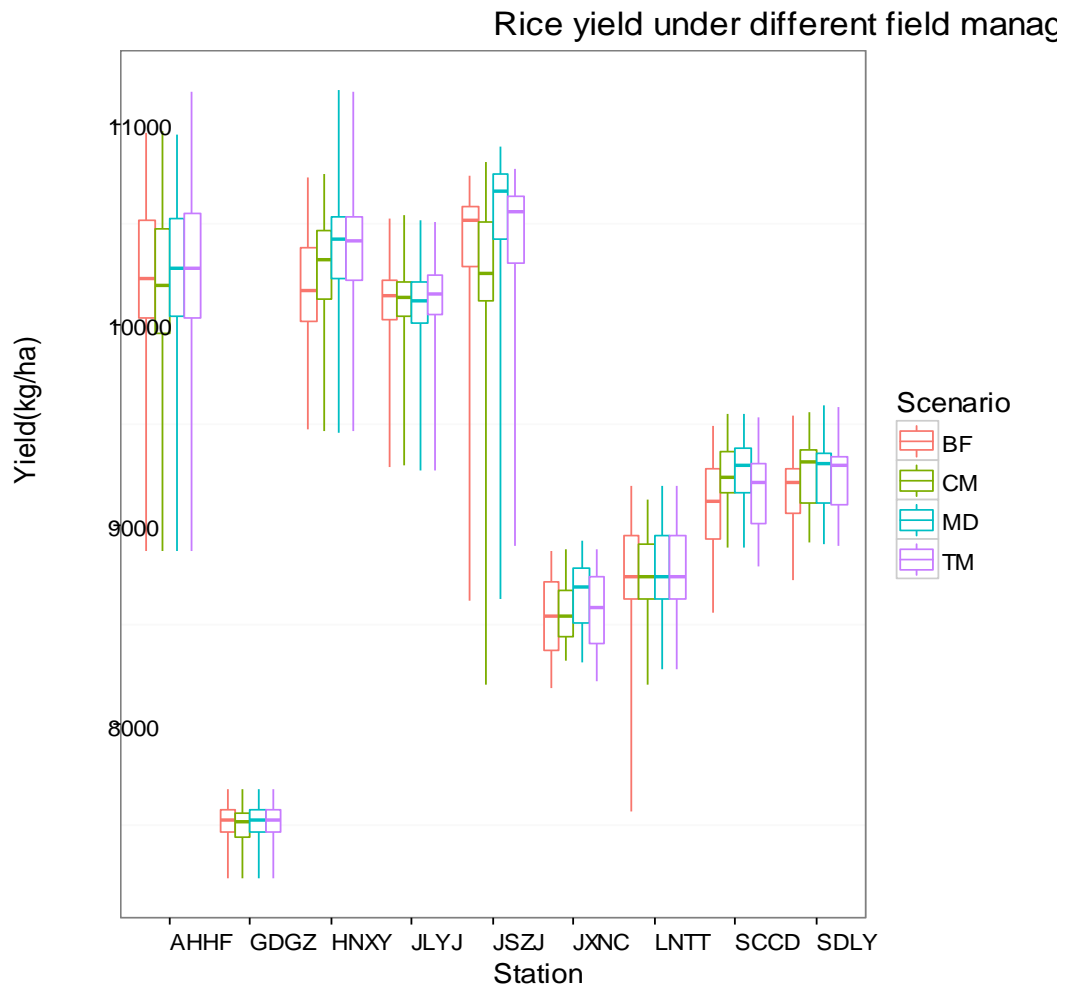
Figure 4. The boxplots of rice yields under field management scenarios of Traditional Management (TM), Balanced Fertilizer (BF), Midseason Drainage (MD) and Comprehensive Management (CM).
