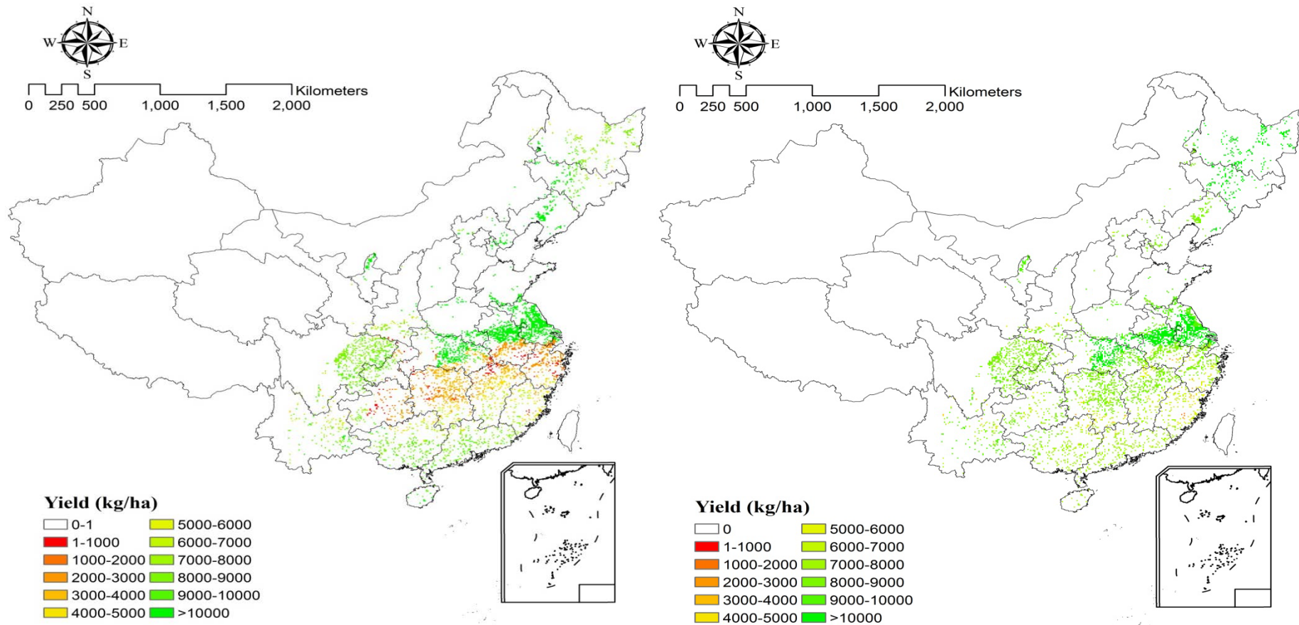
Figure 3. The grid-cell results of rice yield simulation from the original DNDC (left, denoted as Figure 3-a) and coupled DNDC (right, Figure 3-b) model, average over 1981-2010
